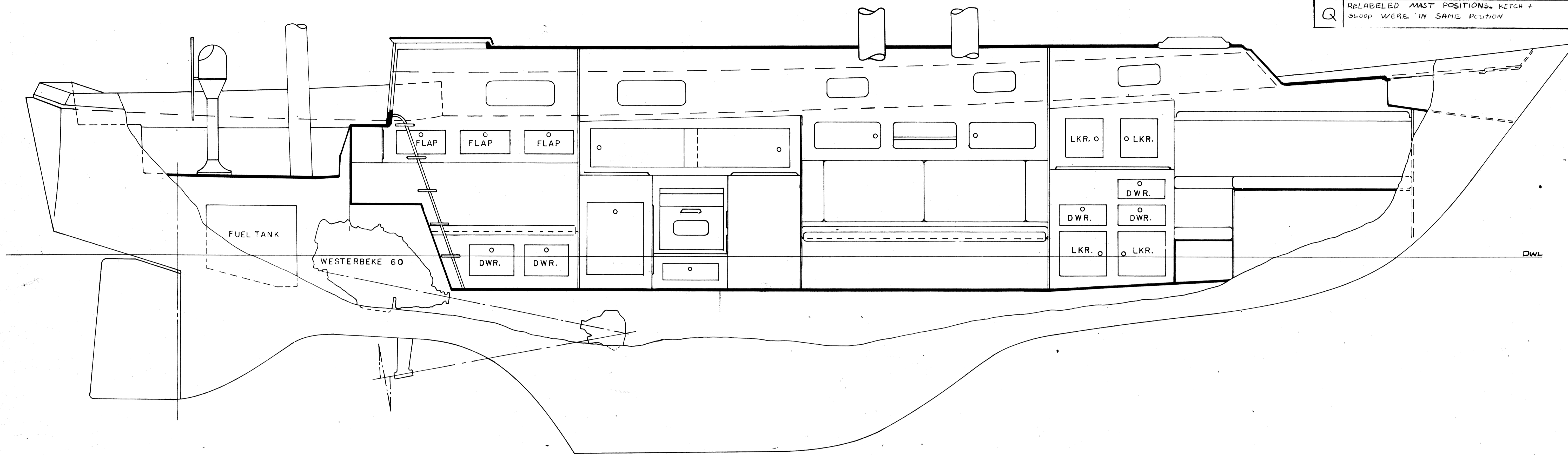
PEARSON 424 HULL 36 AND UP
